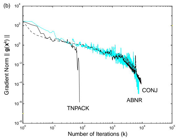
Lysozyme minimization.
