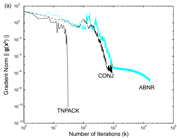
Alanine dipeptide minimization.
